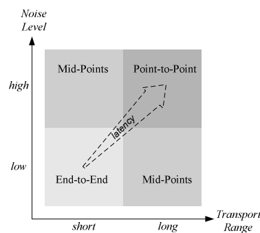
Figure 6. Micro-Modem application types.
