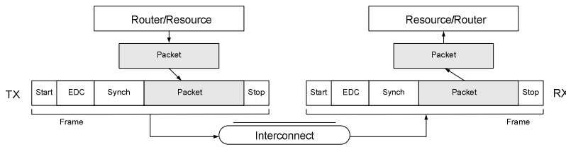
Figure 4. Data transportation scheme
