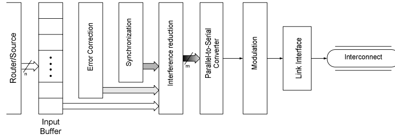
Figure 3. Transmitter architecture in the micro-modem concept
