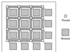
Figure 1. Typical Network on Chip structure.
